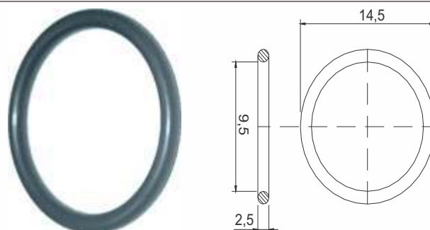
ANEL O'RING DO SNIF
